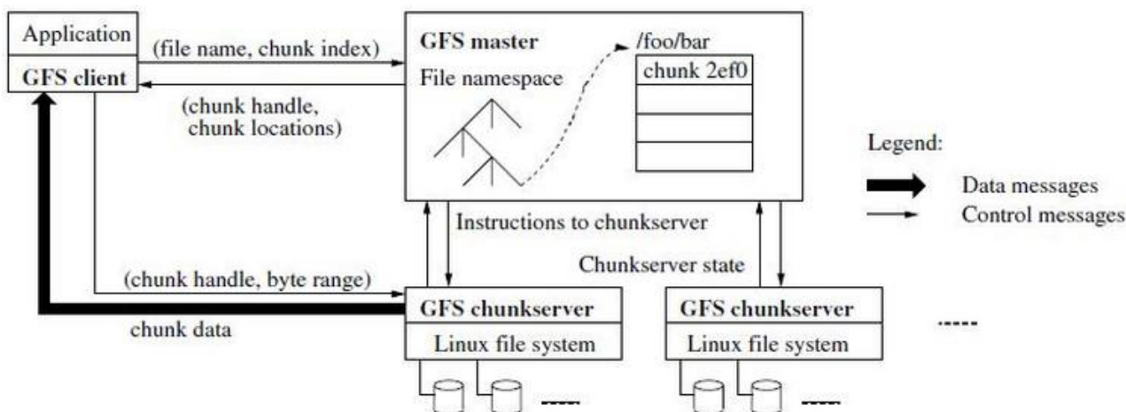
Figure 1: GFS Architecture
