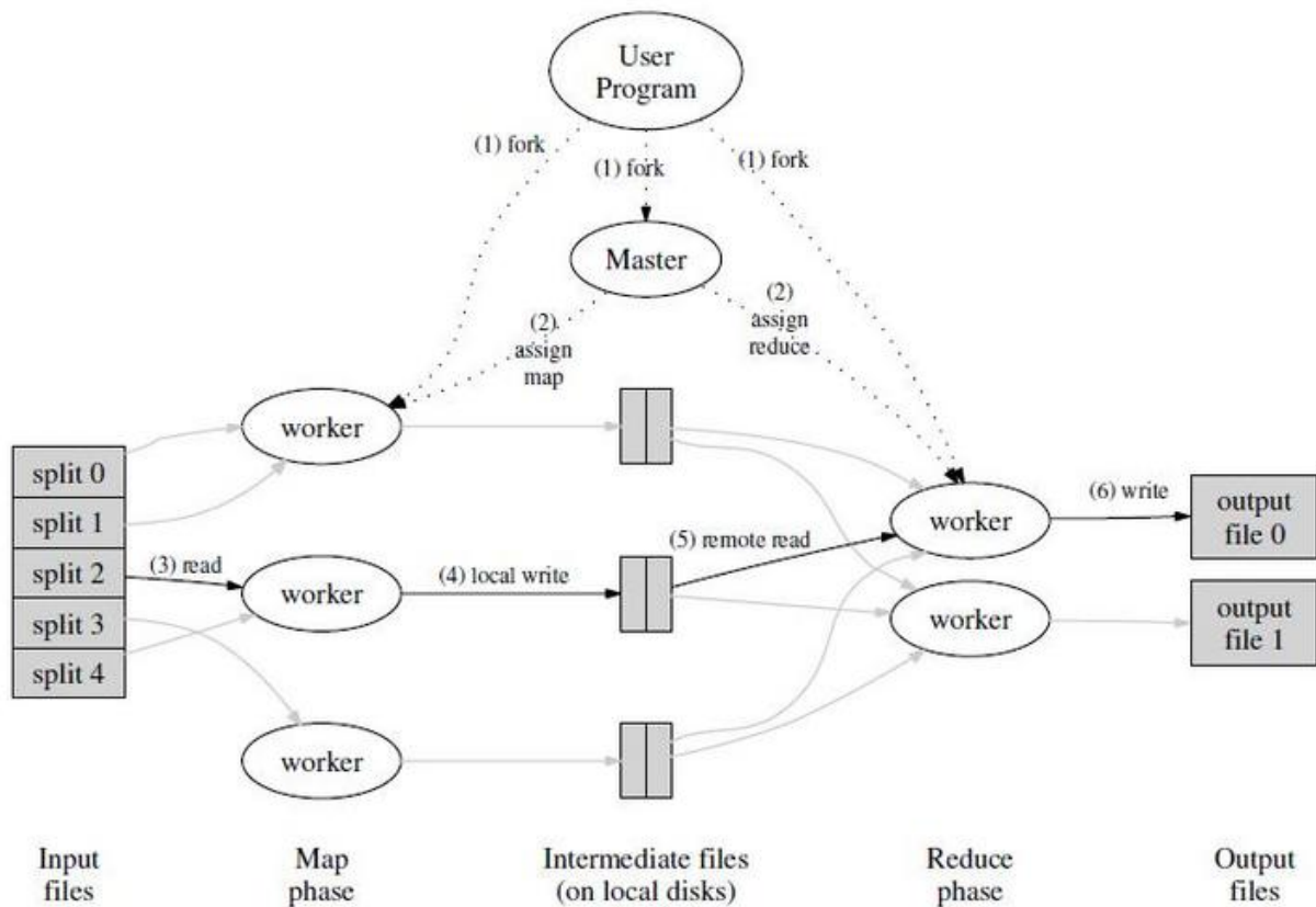
Figure 1: Execution overview
